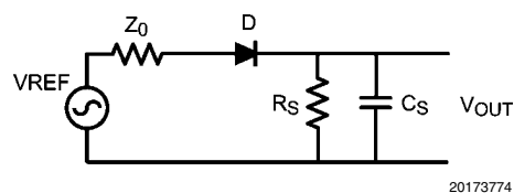
FIGURE 2. Diode Detector
