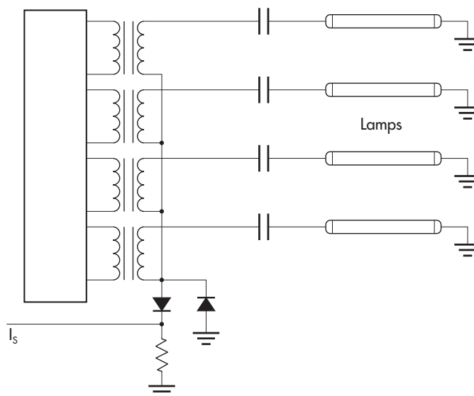
FIGURE 2 — Quad Output Stage
