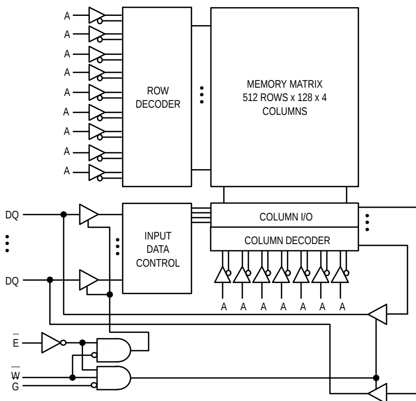
BLOCK DIAGRAM
