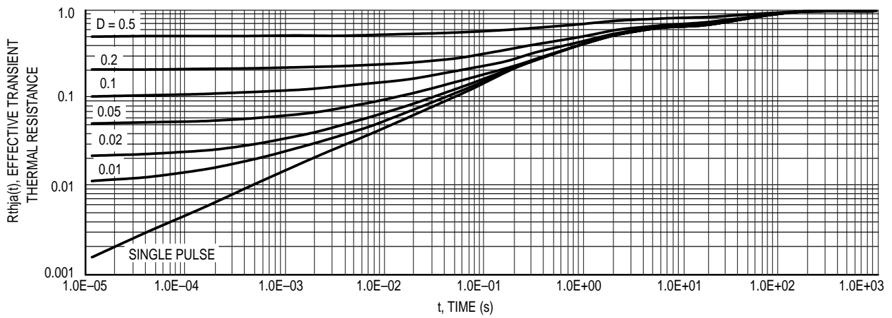
Figure 14. Thermal Response
