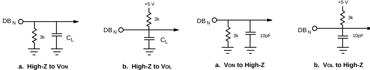
Figure 4. Load Circuit for Bus Relinquish Time Test
