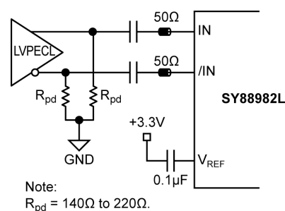
Figure 2b. AC-Coupling to LVPECL Driver
