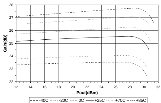
Gain vs Pout F=3.4GHz
