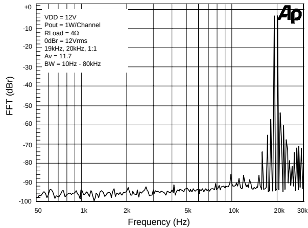
Intermodulation Performance
