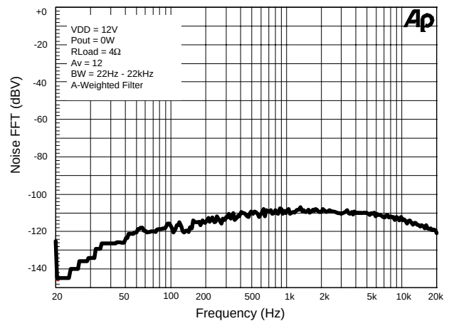
Noise Floor
