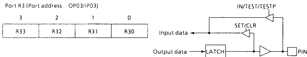
Figure 3-2. Port R3
