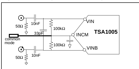
Figure 4: AC-coupled differential input
