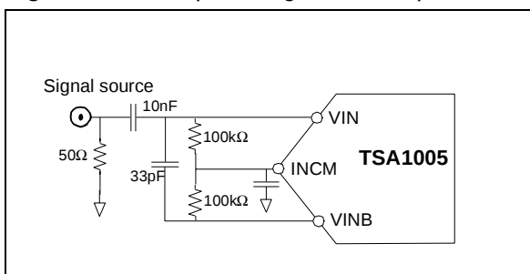
Figure 5: AC-coupled Single-ended input
