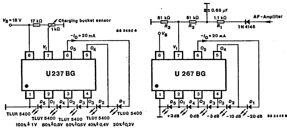
Fig. 4 Liquid level display with linear resistance pickup
