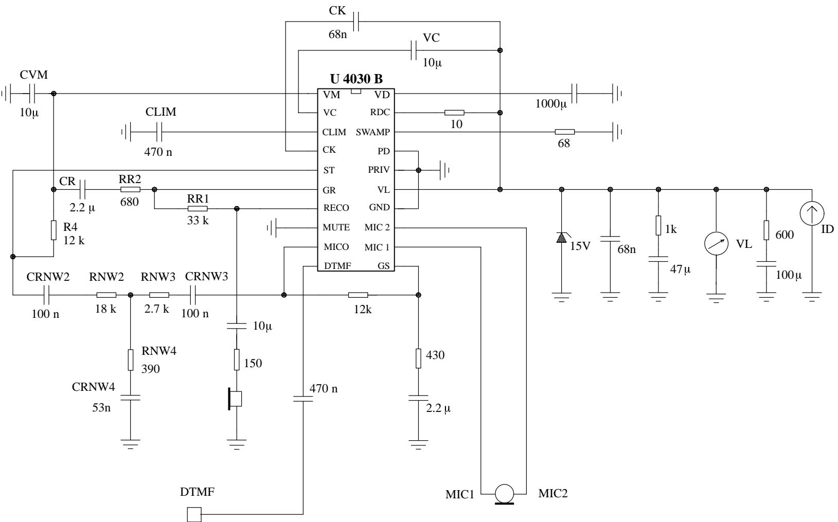
Figure 9. Application Circuit
