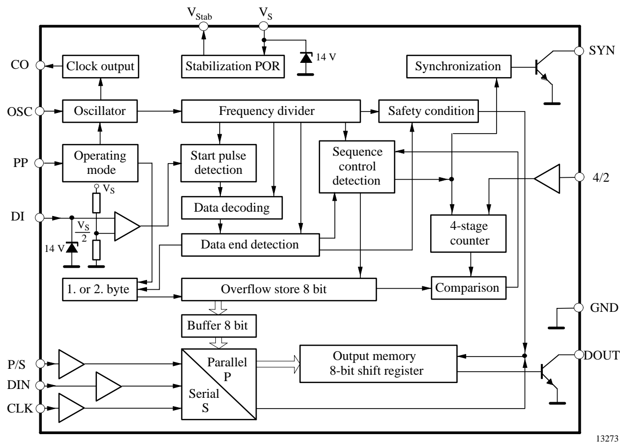
Figure 1. Block diagram
