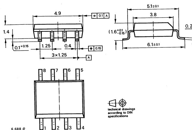
Case S0 8 (SOT 96 A)
