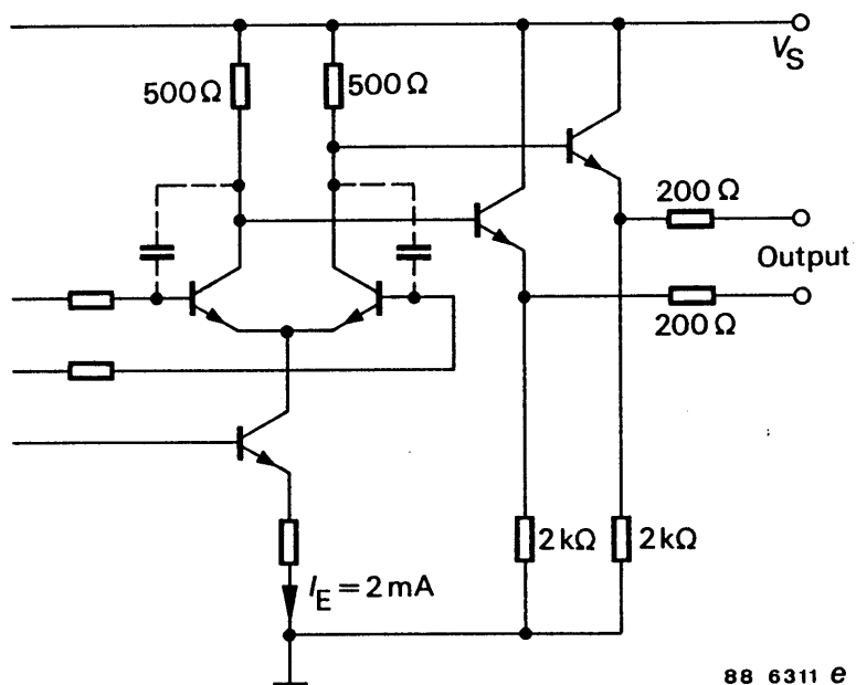
Emitter follower output (U 813 BSE)
