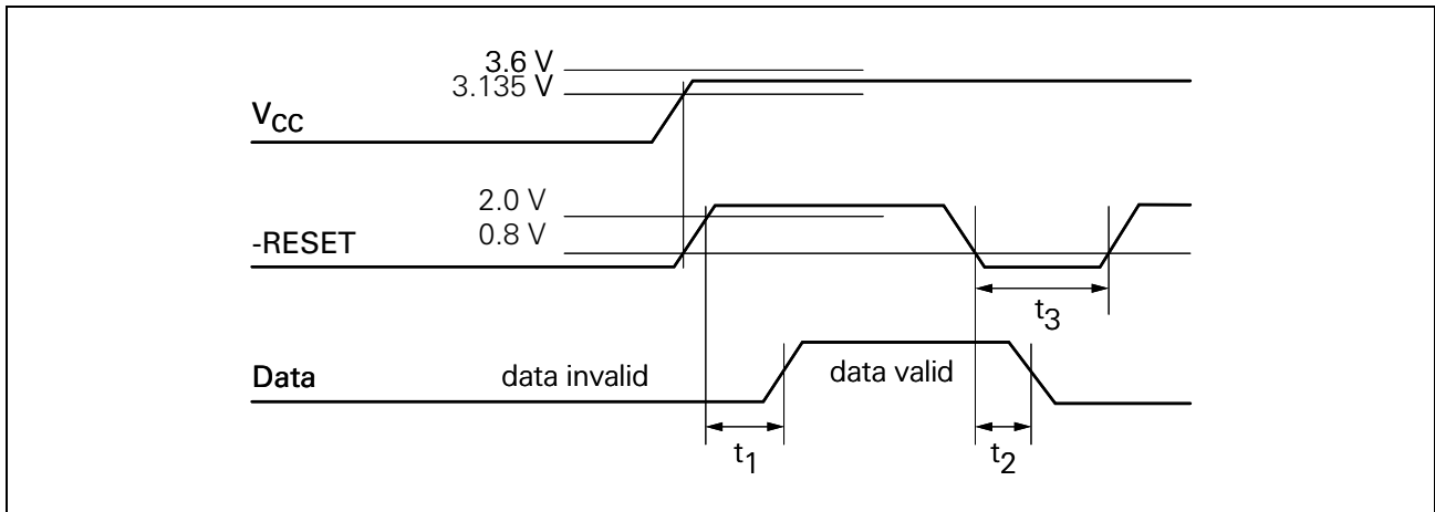
Figure 7 Timing Diagram
