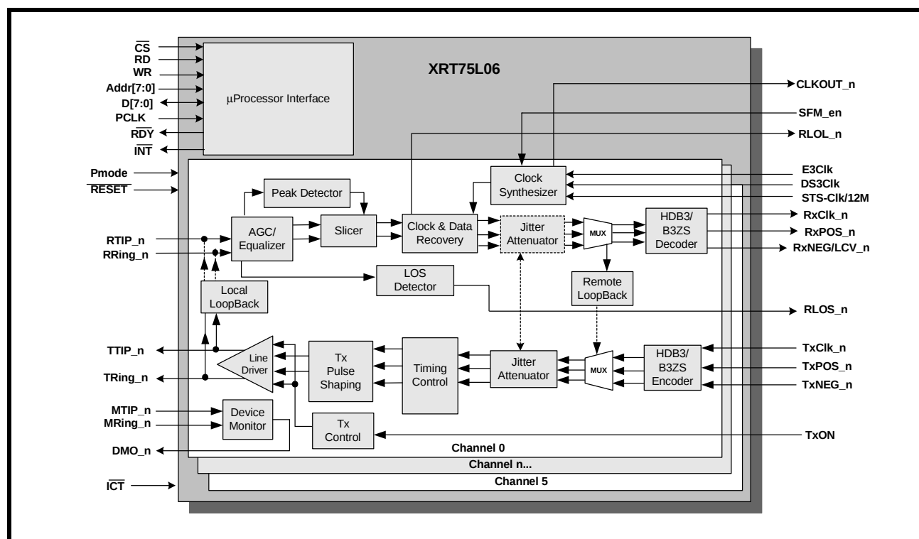
FIGURE 1. BLOCK DIAGRAM OF THE XRT 75L06
