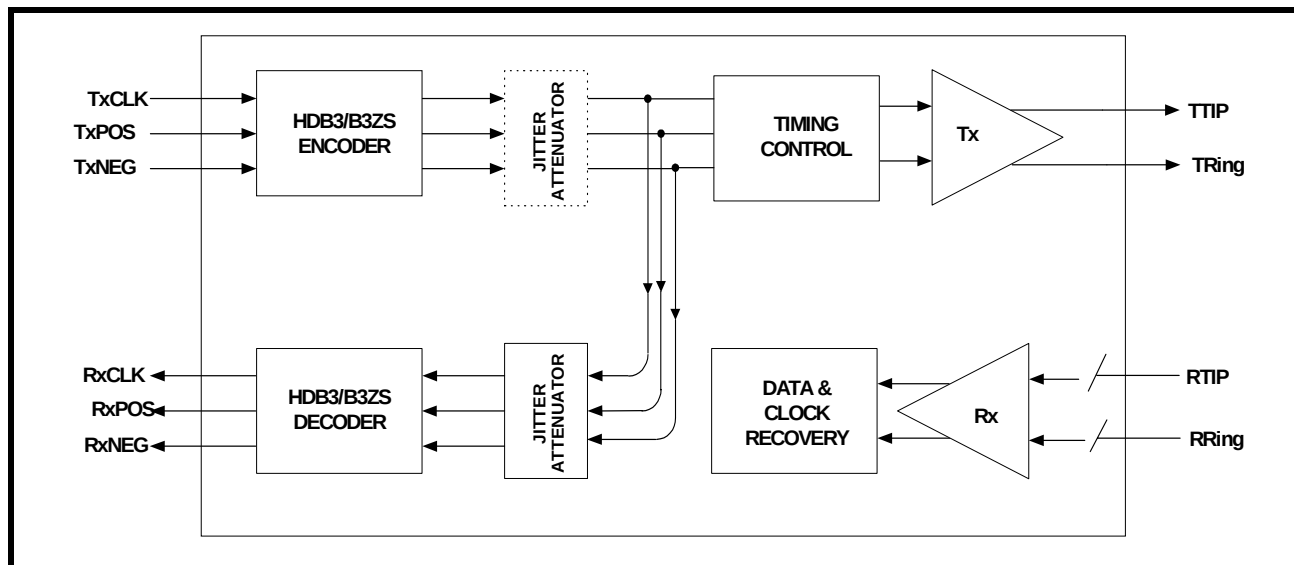
FIGURE 31. DIGITAL LOOPBACK
