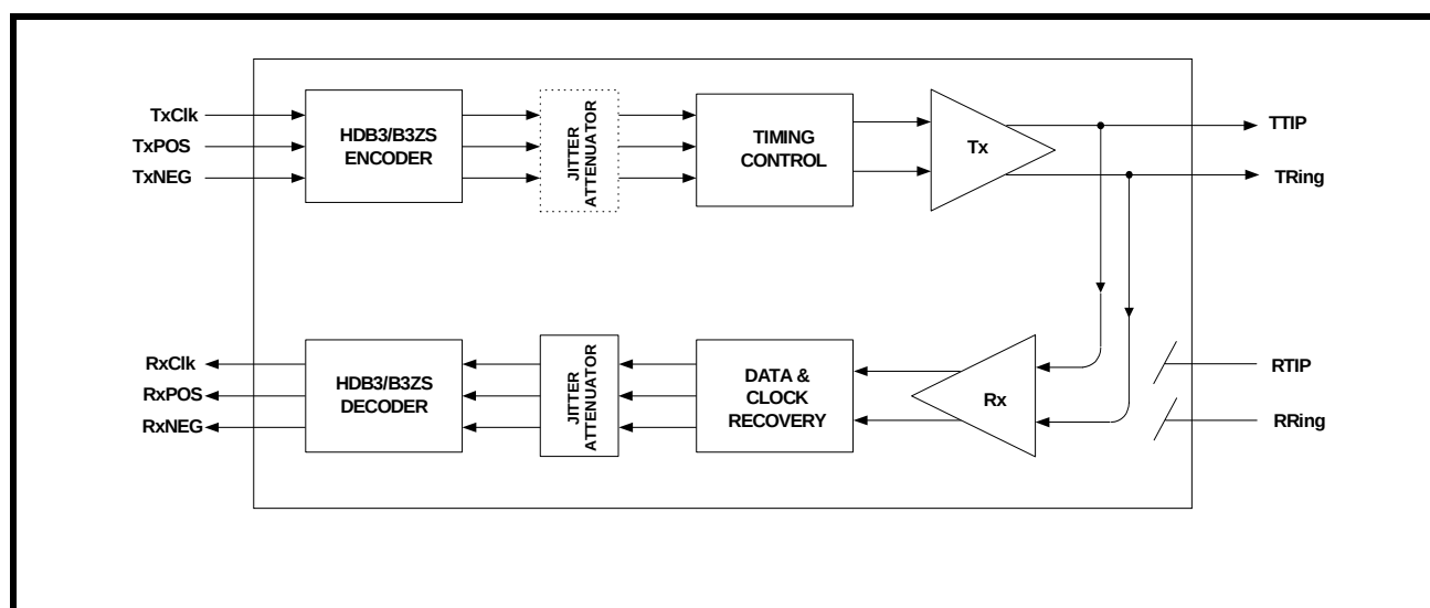
FIGURE 30. ANALOG LOOPBACK
