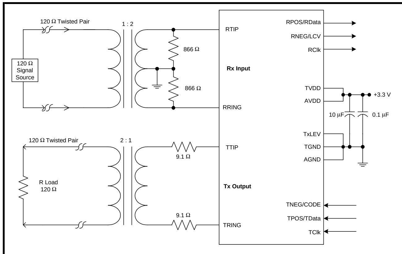
FIGURE 11. ILLUSTRATION OF HOW TO INTERFACE THE XRT82D20 TO THE LINE FOR 120 \Omega APPLICATIONS AND 3.3V OPERATION ONLY
