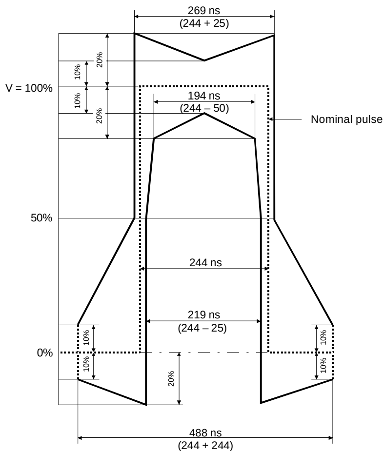
FIGURE 9. ILLUSTRATION OF THE ITU-T G.703 PULSE TEMPLATE FOR E1 APPLICATION
