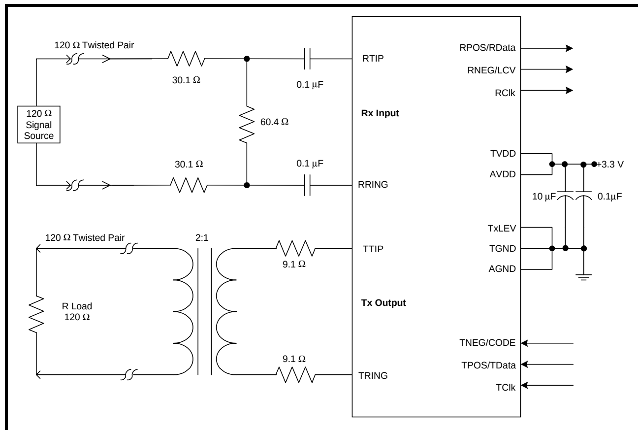
FIGURE 15. CAPACITIVELY-COUPLING THE RECEIVE SECTION FOR 120 \Omega APPLICATION AND 3.3V SUPPLY
