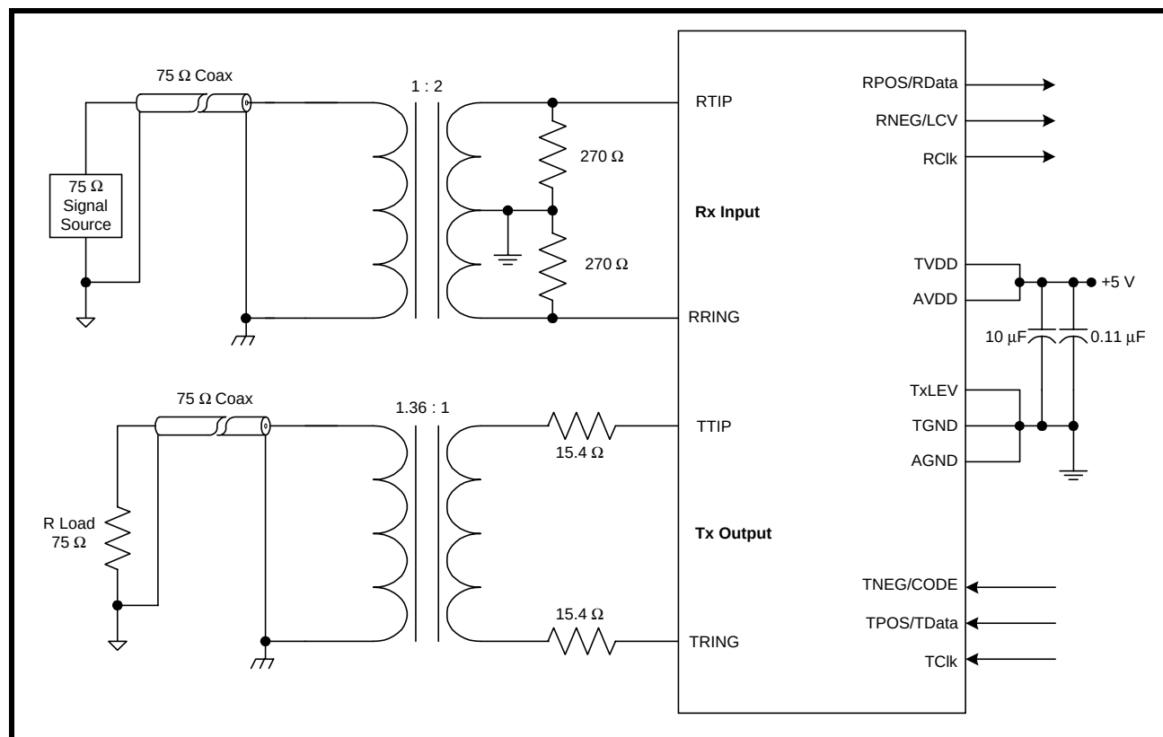
FIGURE 12. RECOMMENDED SCHEMATIC FOR TRANSFORMER-COUPPLING THE XRT82D20 TO THE LINE FOR 75 \Omega APPLICATIONS AND 5 V OPERATION ONLY
