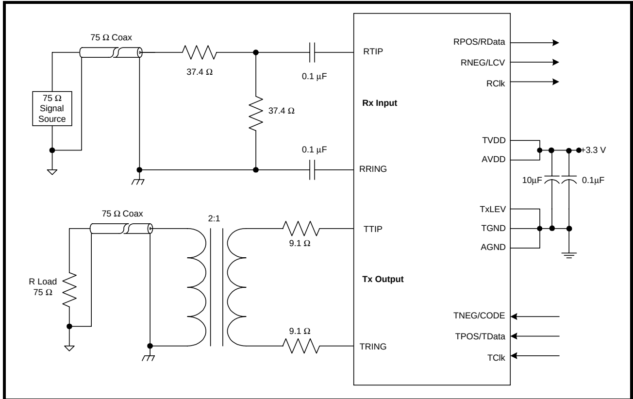
FIGURE 14. CAPACITIVELY-COUPLING THE RECEIVE SECTION FOR 75 \Omega APPLICATION AND 3.3V SUPPLY
