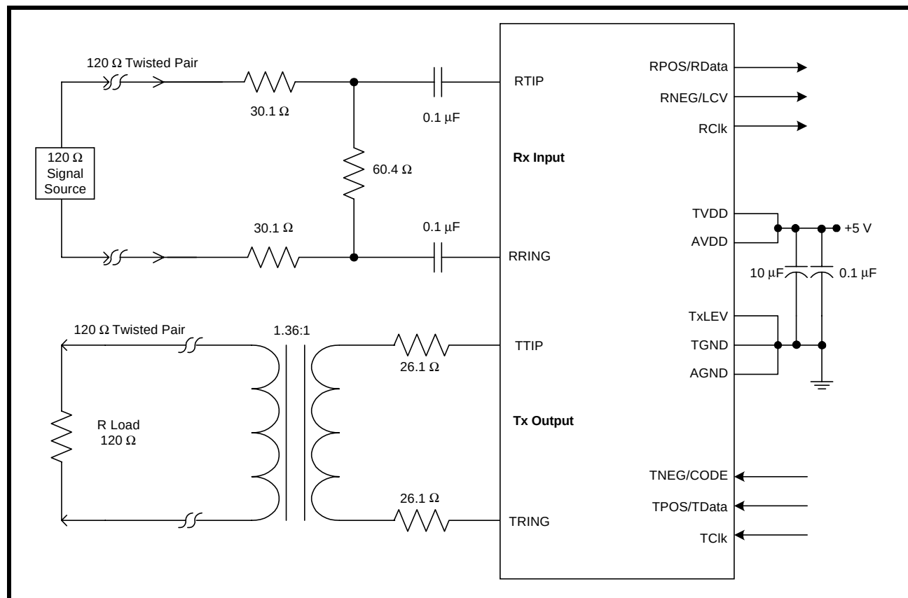
FIGURE 17. CAPACITIVELY-COUPLING THE RECEIVE SECTION FOR 120 \Omega APPLICATION AND 5V SUPPLY
