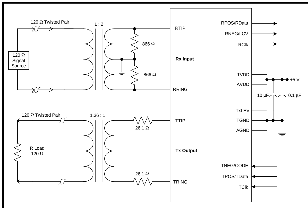
FIGURE 13. RECOMMENDED SCHEMATIC FOR TRANSFORMER-COUPLING THE XRT82D20 TO THE LINE FOR 120 \Omega APPLICATIONS AND 5 V OPERATION ONLY
