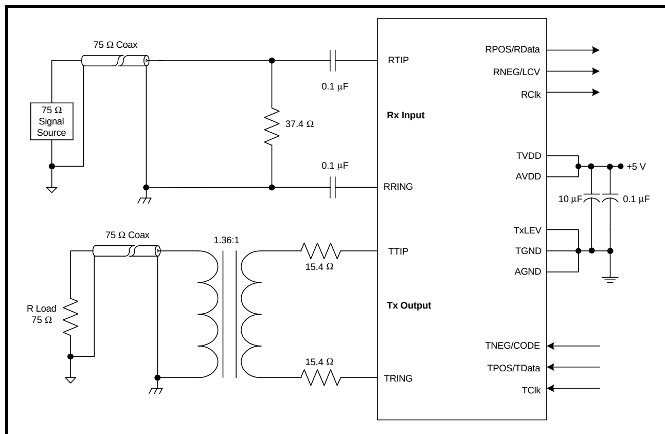
FIGURE 16. CAPACITIVELY-COUPLING THE RECEIVE SECTION FOR 75 \Omega APPLICATION AND 5V SUPPLY
