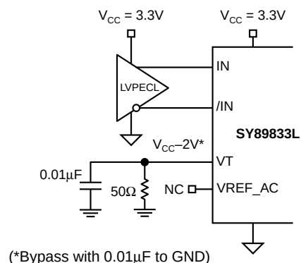
Figure 3c. DC-Coupled PECL Input Interface
