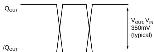
Figure 2c. Single-Ended Swing
