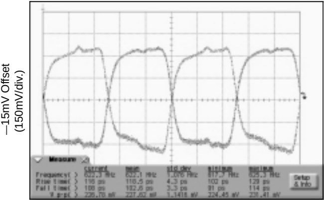
622MHz Output
