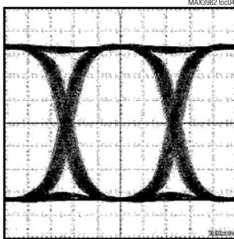
END-TO-END EYE DIAGRAM, 20m 24AWG CABLE AT 4.25Gbps
