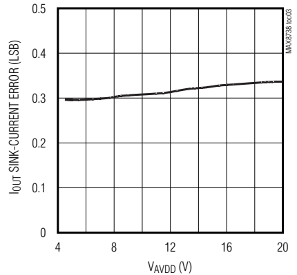
I OUT SINK-CURRENT ERROR vs. V AVDD
