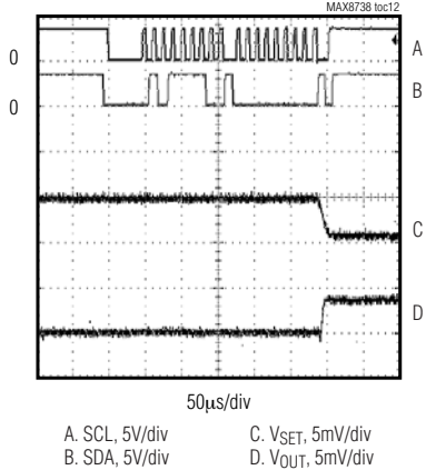
SINGLE LSB STEP-DOWN RESPONSE
