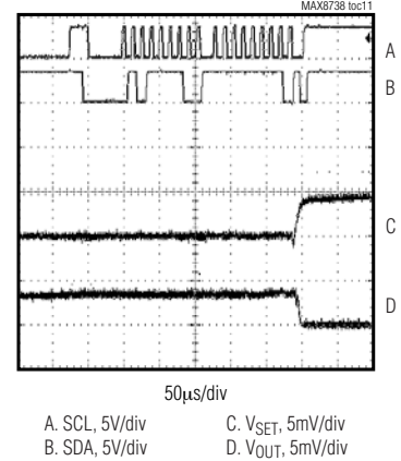
SINGLE LSB STEP-UP RESPONSE
