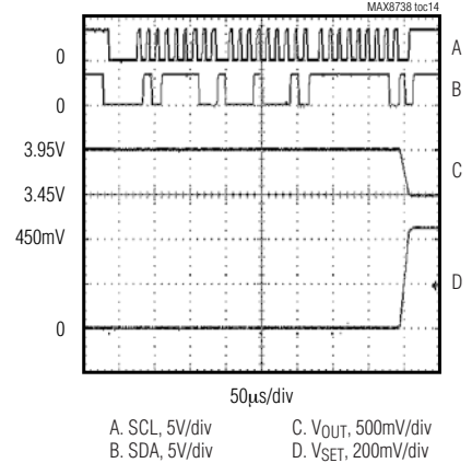
WRITE FFH RESPONSE
