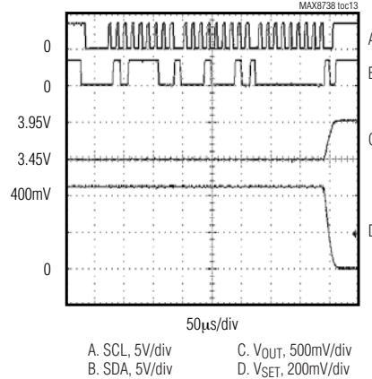
WRITE 00H RESPONSE
